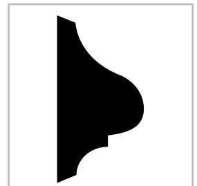
Panel Mould 183 Solid Pine 9/16 x 1-1/8
