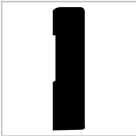
Casing 473 (R2E) MDF 5/8 x 2-1/4
