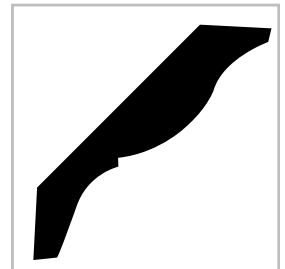
Crown C22 Pine 11/16 X 3-5/8
