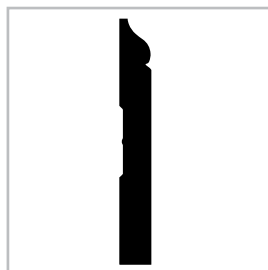
Baseboard 665 Primed Pine 9/16 x 3-15/16
