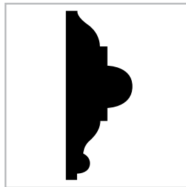
Chair Rail 300 Primed Pine, MDF 1-1/16 x 3
