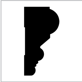
Chair Rail C43 Primed Pine 1-1/4 x 2-1/2
