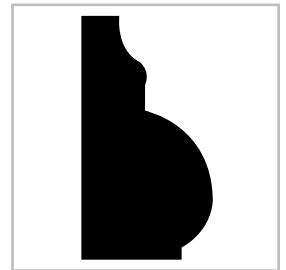
Base Cap 113 Solid Pine 11/16 x 1-1/4
