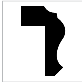
Ply Cap 292 Solid Pine 5/8 x 1-1/8
