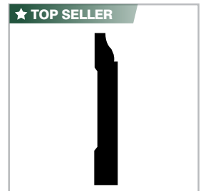
Baseboard 623 Pine, FJ Pine, MDF, Primed Pine 9/16 x 3-1/4
