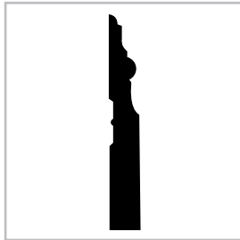
Baseboard 9243 MDF 11/16 x 5-1/4
