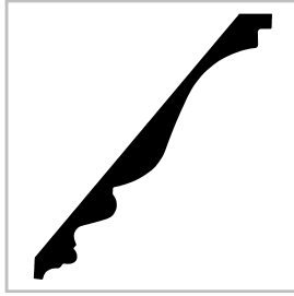
Crown 270 MDF 18mm x 6-3/4
