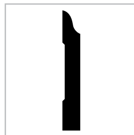
Baseboard 663 Pine, Primed Pine, MDF 9/16 x 3-1/4
