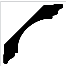
Crown 41 MDF 30mm x 6-5/16
