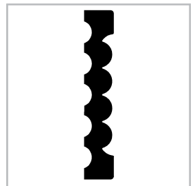
Casing 908 MDF 9/16 x 3-1/4
