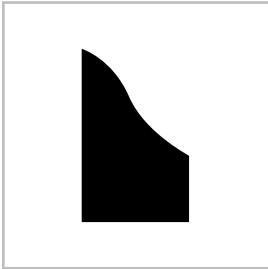
Base Shoe 131 Primed Pine, Oak 7/16 x 11/16
