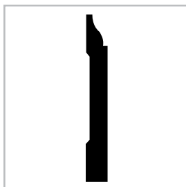
Baseboard 622 Primed Pine, MDF 1/2 x 3-1/2
