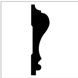
Chair Rail 390 Primed Pine, MDF 11/16 x 2-5/8
