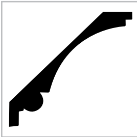
Crown 792 MDF 1-3/16 x 7-3/16
